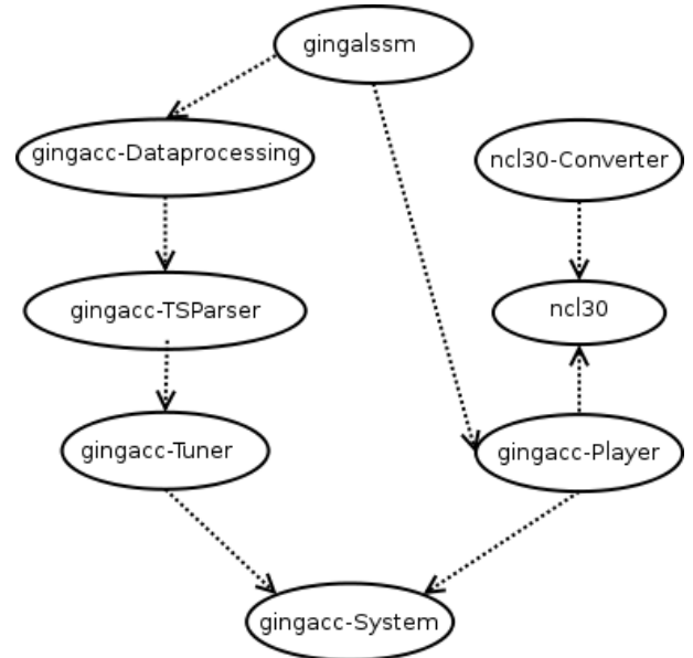
Figure 1: GingaNCL-PUC modules and relationships.
